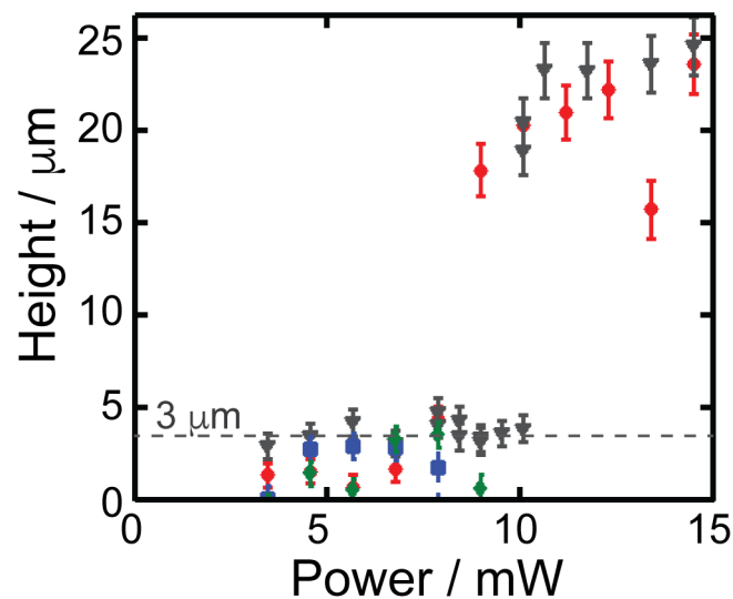
Figure S3. Axial displacement (height) of Au-silica Janus particles (diameter = 1.3 \pm 0.1 \mu\text{m} ) tethered to a glass substrate with a 3 \mu\text{m} in length dsDNA molecule. The different symbols represent the axial displacement behavior for individual DNA-tethered Janus particles. The blue and green data set corresponds to cases where the DNA-tether ruptured before being fully stretched and then the particle fell out of the optical trap.
