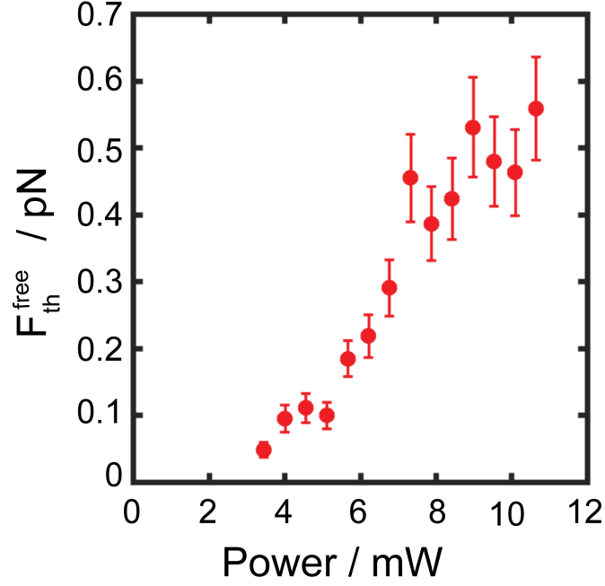
Figure S4. Thermophoretic force acting on free Au-silica Janus particles as a function of the trapping laser power.
