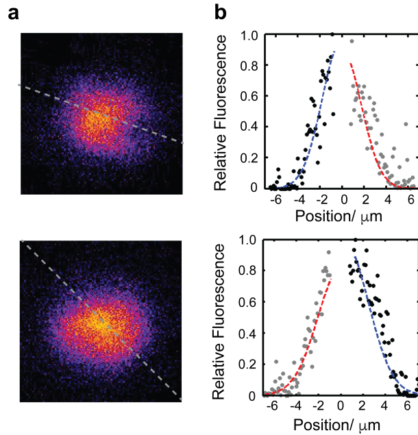
Figure S5. (a) Fluorescence distribution of red fluorescent protein around an optically trapped Au-silica Janus particle. The red fluorescence protein acts as an in-situ temperature sensor and it is excited using an expanded 532 nm laser that is superimposed to the 1064 nm trapping beam. The upper and bottom images correspond to two different rotational orientations of the Janus particle inside the optical trap. The dimensions of the images are 15.7 \times 15.7 \mu\text{m}^2 . The power outputs (and power densities) of the green and IR laser beams are 0.4 ( 1 \mu\text{W}/\mu\text{m}^2 ) and 3.5 mW ( 200 \mu\text{W}/\mu\text{m}^2 ), respectively. (b) Normalized fluorescence intensity profiles of red fluorescence protein across the grey dashed lines presented in a. The fluorescence signal over the Janus particles was discarded. The dashed lines correspond to the Gaussian fits of the experimental data around the silica (blue) and gold-coated (red) hemispheres of the Janus particle.
