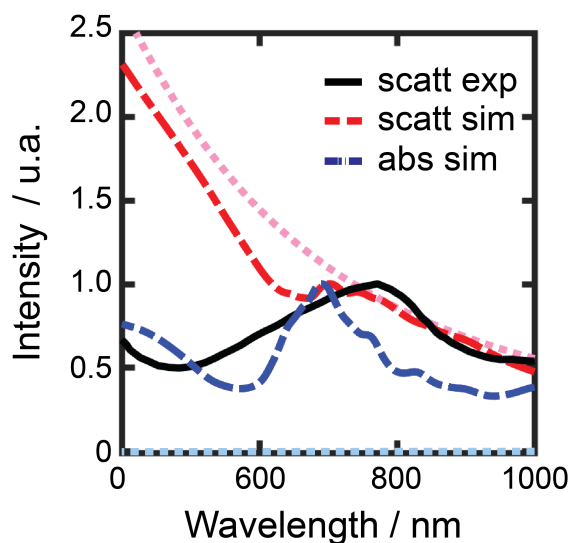
Figure S1. Simulated scattering (red dashed line) and absorption (blue dashed line) spectra of an individual 1.3 \mu\text{m} in diameter Au-silica Janus particle with a 5 nm thick gold half-coating in water. Representative white light scattering spectrum of an individual Au-silica Janus particle in water measured experimentally (black solid line). Simulated scattering (pink dotted line) and absorption (light-blue dotted line) spectra of an individual 1.3 \mu\text{m} in diameter bare silica sphere in water.
