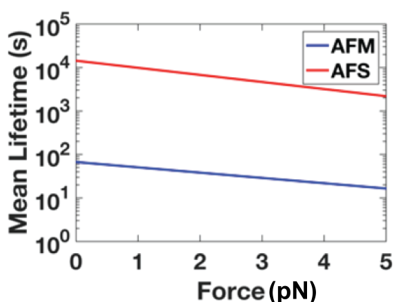
Figure S7. Mean lifetime of DIG-antiDIG bond as a function of the applied force. The plot was generated using the results of Wuite and coworkers 10 and Gaub and coworkers 11 who measured the DIG-antiDIG bond lifetime using acoustic force spectroscopy (AFS) and atomic force microscopy (AFM), respectively.
