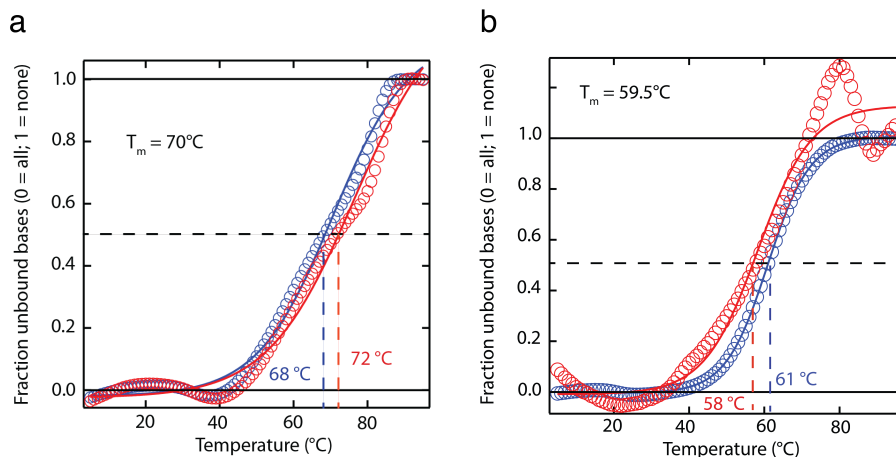
Figure S6. Melting curve for the 9-kb-long dsDNA construct used for Janus particle-based stretching experiments. The data corresponds to the fraction of “unpaired bases” as a function of the temperature. Blue and red illustrate the data recorded going down from 95 to 5 °C and up from 5 to 95 °C, respectively. The presence of some hysteresis in the data is explained by
