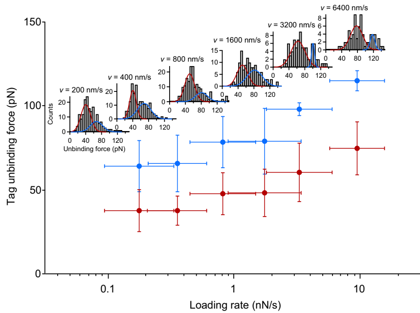
Fig. S3. Tag unbinding forces as a function of the applied loading rate. Tag unbinding represents the dissociation of the Twin-Strep-tag from tetravalent Strep-Tactin. Mean forces were obtained by fitting a bimodal Gaussian function to the distribution of unbinding forces for each pulling speed. Loading rates were obtained by fitting a line to force-extension traces before the last peak. Mean values of loading rates were obtained by fitting a Gaussian to the loading-rate distributions for each pulling speed. Error bars are 1 SD. Force-loading-rate dependency and bimodality of the individual force distributions are in line with previous investigations of the specific Strep-tag/Strep-Tactin interaction (27).
