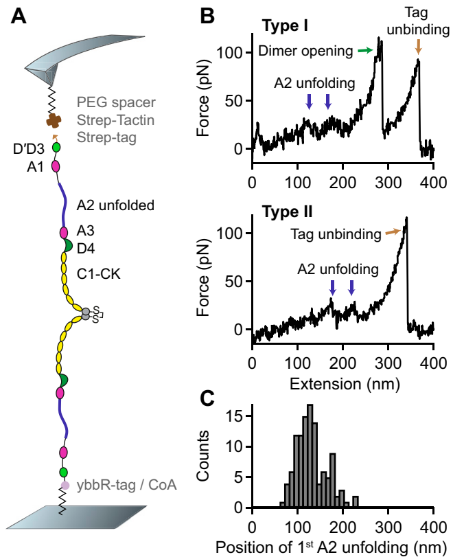
Fig. S4. Single-molecule force measurements on VWF heterodimers carrying a single Strep-tag instead of a Twin-Strep-tag. (A) Schematic representation of the pulling configuration. (B) Denoised force-extension traces. Traces of type I and II were still observed. (C) Bimodal distribution of the position of the first A2 unfolding event.
