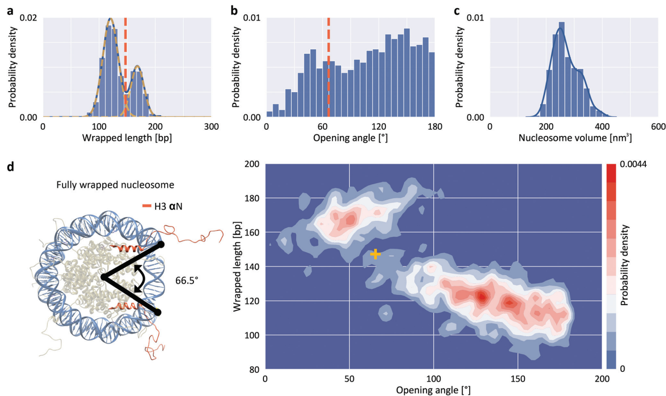
Fig. 2 Structure parameters for H3 nucleosomes from AFM imaging. a, Wrapped DNA length distribution fitted using the sum of two Gaussians (centered at 120 \pm 14 bp and 168 \pm 12 bp). b, DNA opening angle distribution. The dashed orange line indicates the expected position of a fully wrapped nucleosome. c, Nucleosome core particle volume distribution. The solid line is a kernel density estimate. d, 2D kernel density profile (bandwidth = 2.5^\circ , 2.5 bp) of nucleosome opening angle and wrapped length. The expected position of fully wrapped nucleosomes based on the crystal structure (left; rendered from PDB 1KX5) is shown as a yellow cross at an opening angle of 66.5^\circ and a wrapped DNA length of 147 bp. The data set shown includes N = 1011 nucleosomes.
